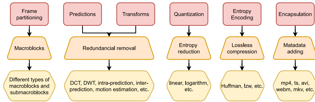
Fig. 1. Main steps of video encoders.
